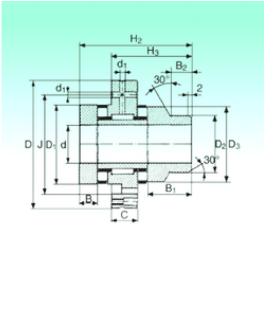
ZARF 55145 L TN Bearing 2D drawings and 3D CAD models
