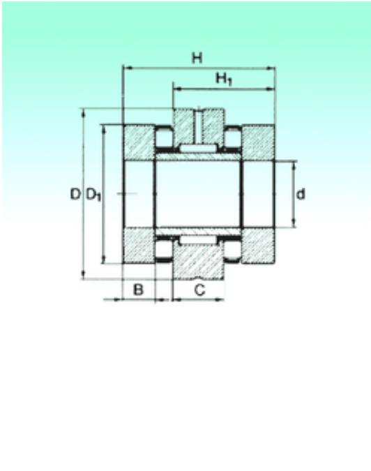
ZARN 65125 TN Bearing 2D drawings and 3D CAD models
