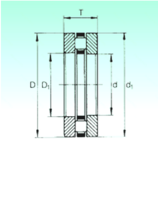
81168 Bearing 2D drawings and 3D CAD models
